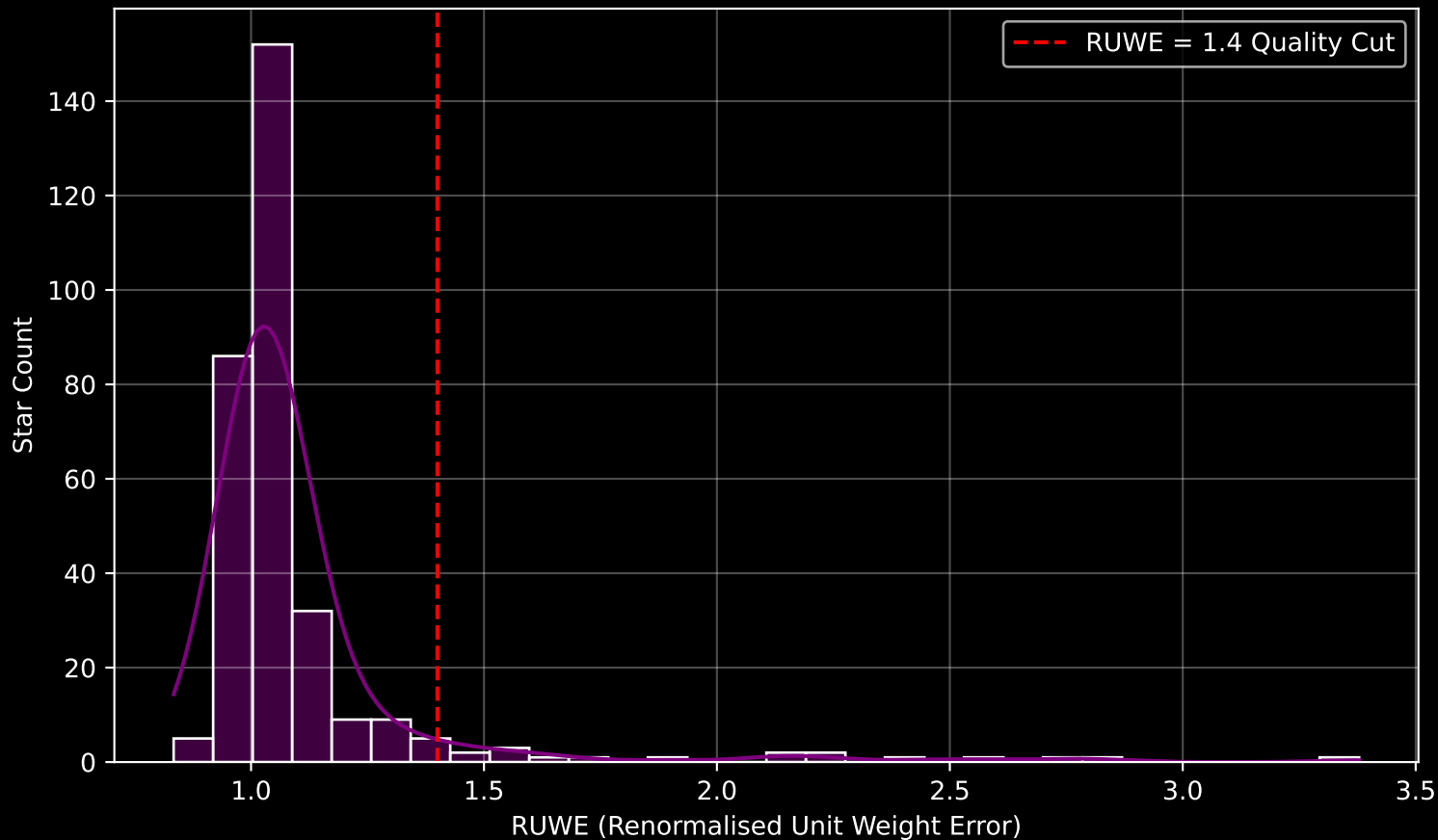
GAPOGEE DR17 Field [191-12] RUWE Distribution (n= 315)
