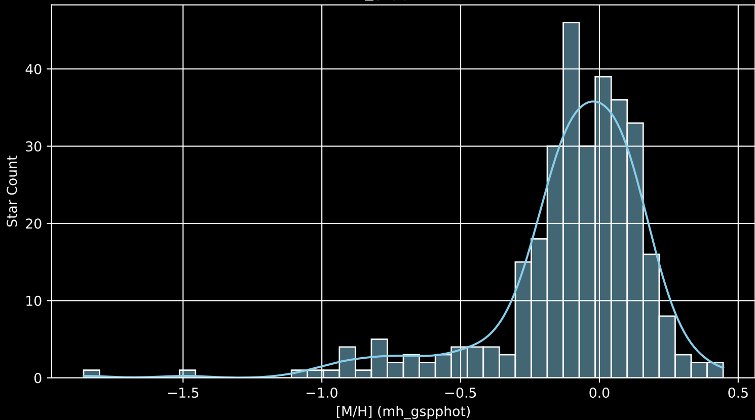
APOGEE DR17 Field: [191-12 [M/H] (mh_gspphot) (n= 318)
