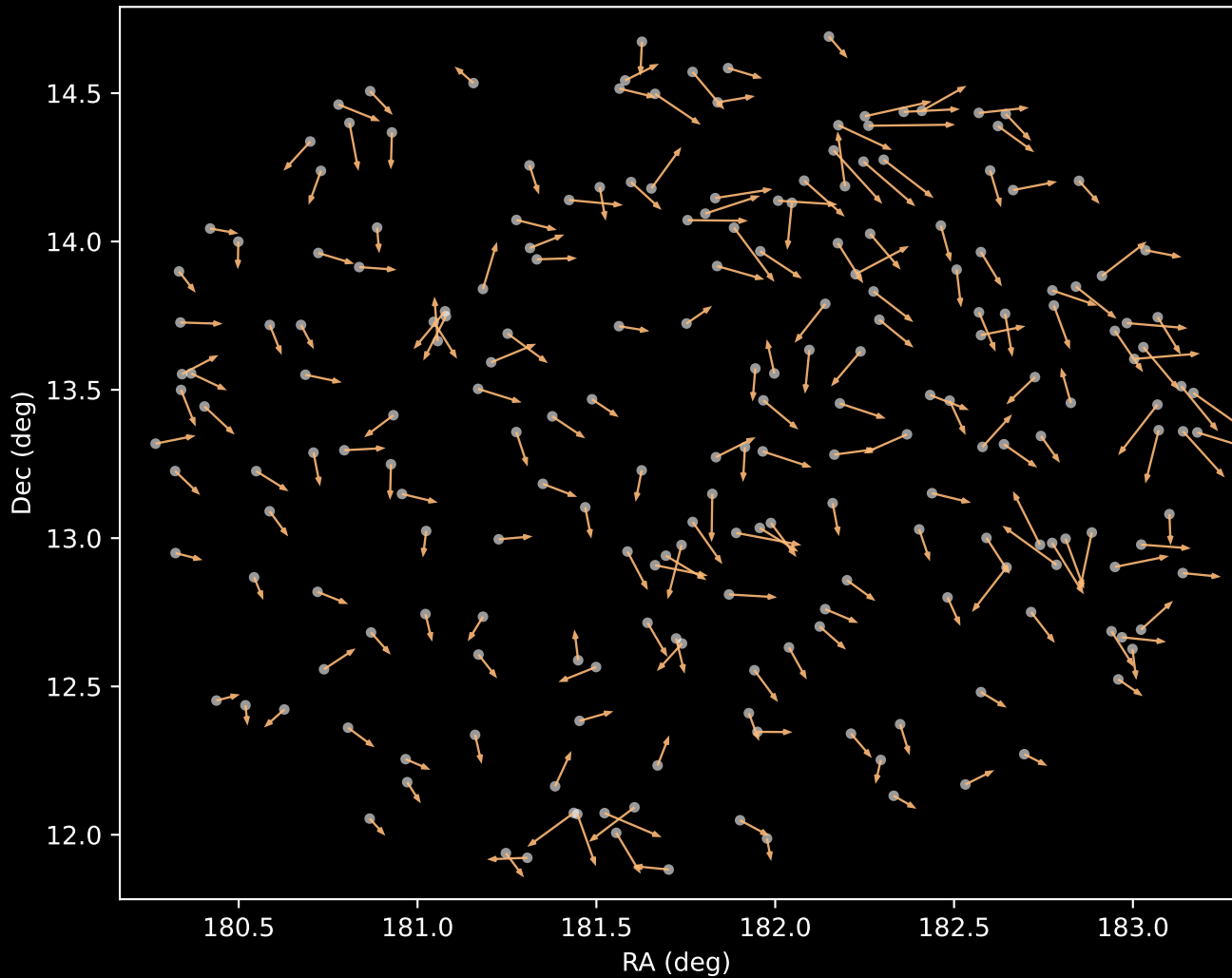
APOGEE DR17 Cluster 3 Proper Motion Vectors (n=213)
