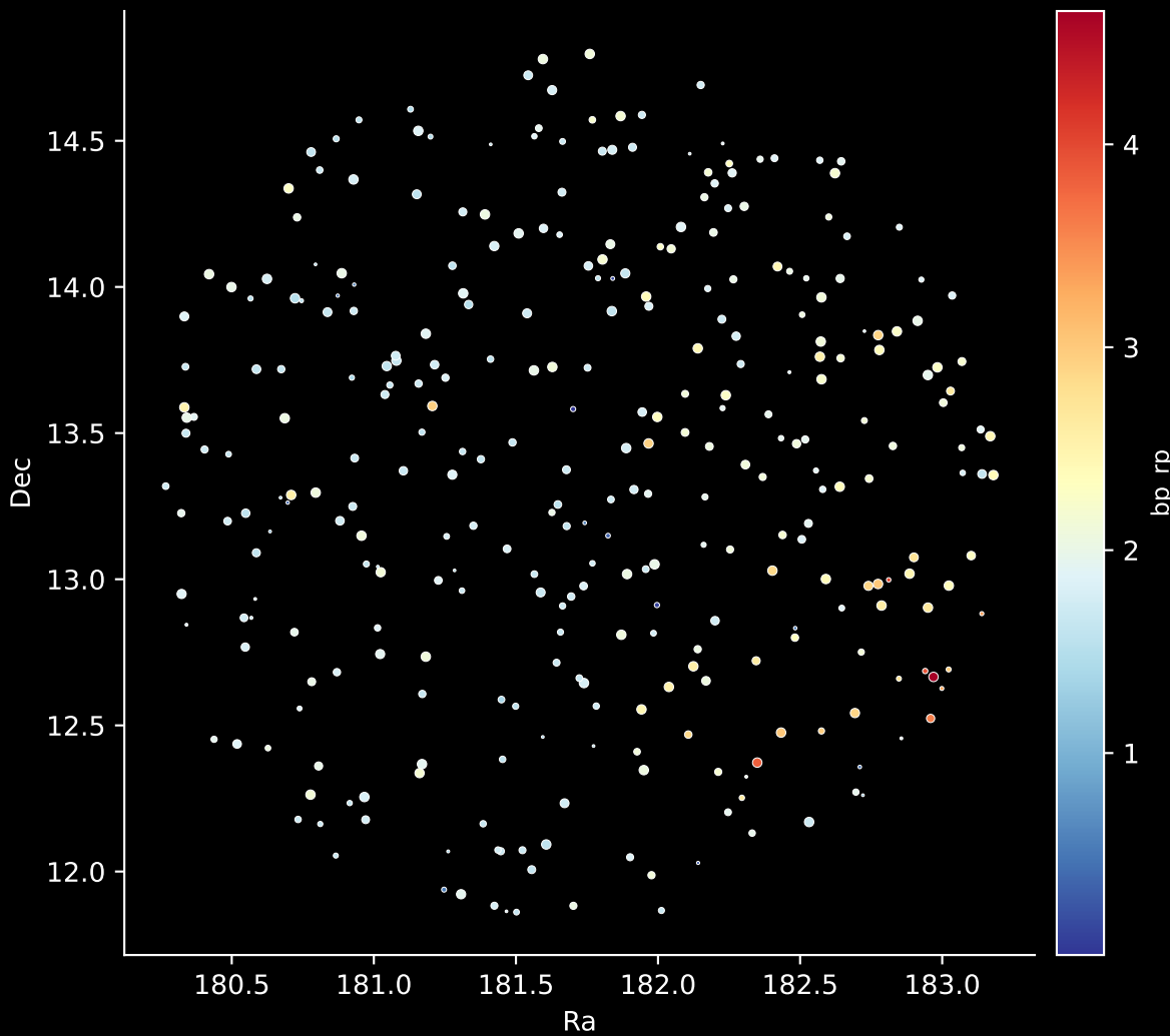
APOGEE DR17 Field: [191-12] Stars: 319
