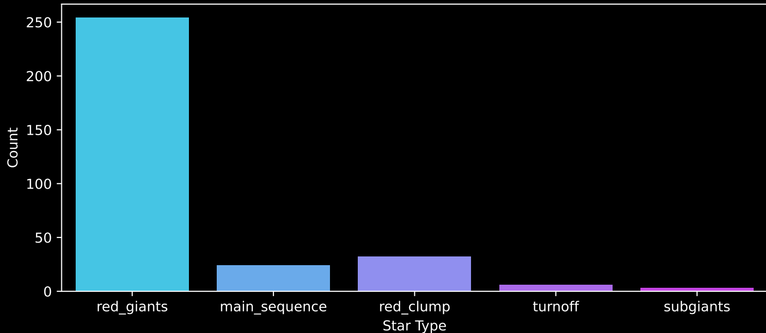
APOGEE DR17 Field: [191-12] Count plot of Star Type
