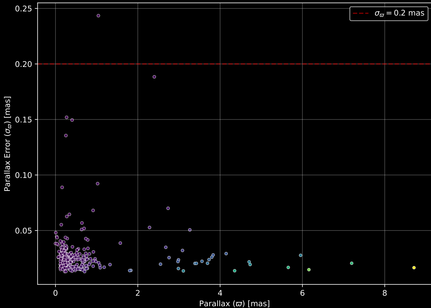
APOGEE DR17 Field: [191-12] Parallax Quality (n= 319)
