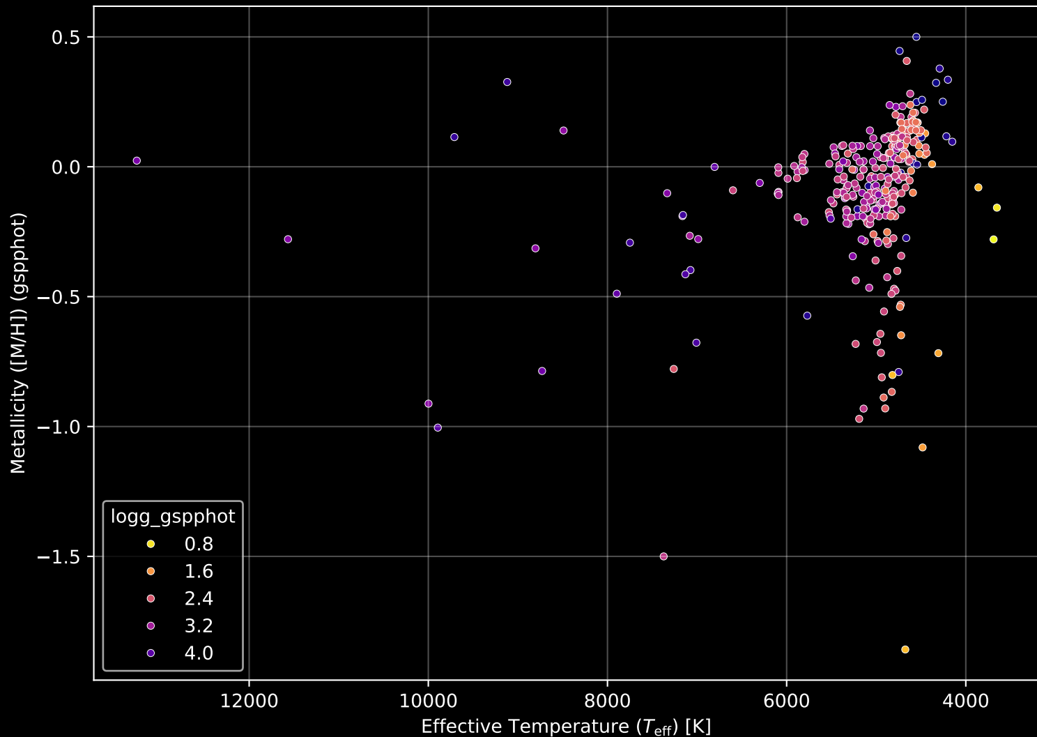
APOGEE DR17 Field: [191-12] Stellar Population Parameters (n= 319)
