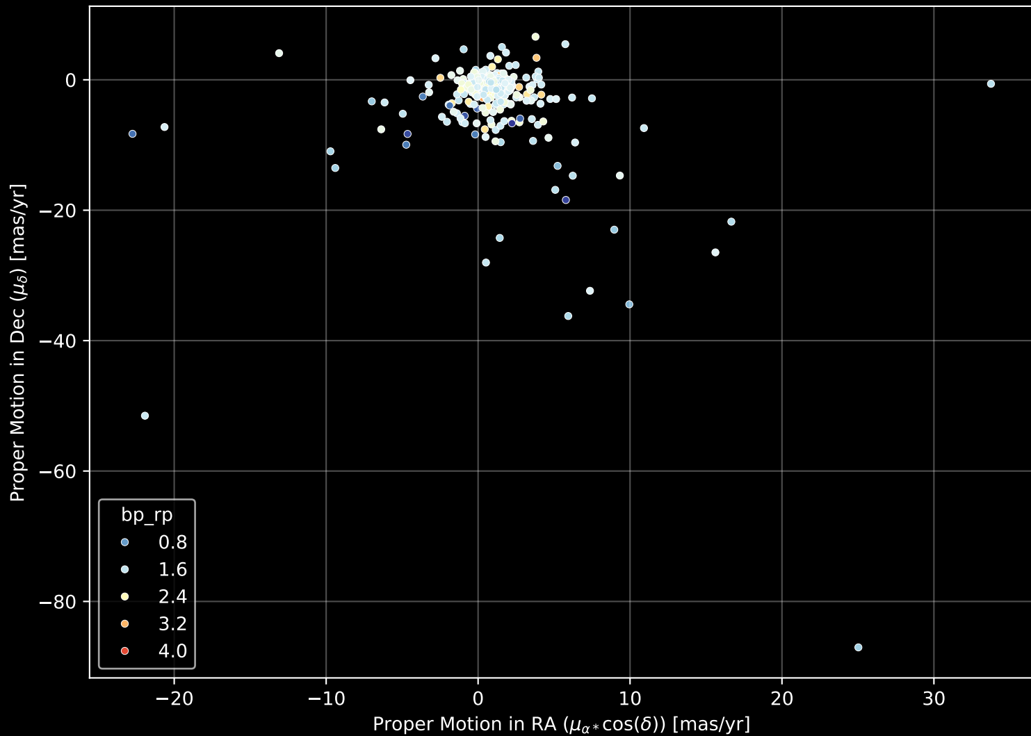
APOGEE DR17 Field: [191-12] Proper Motion Diagram (n= 319)
